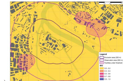
Fig. 2. Vulnerability representation of natural hazards not significant to the industrial context. a) Wildfires (IBO). b) Earthquakes (SIS).
